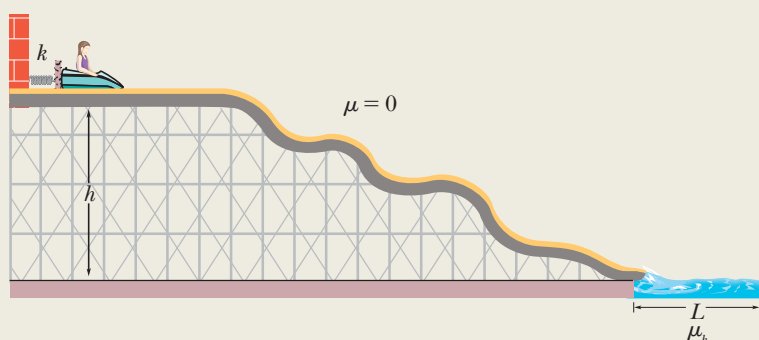
Figure 8-17 A spring-loaded amusement park water slide.
